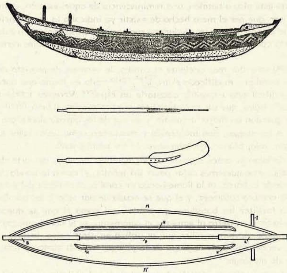
B Arekin, ( Carillo de proa ), Dalhuta o truban, ( quilla o erboix ). II: Iatrobai ( Caremas ) I. Iatrokan ( Eragunde ) L. alkoch ( Roda de proa ) N, osdar ( Ertridor ) N'almankab ( Babor )
